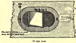
Mode of mounting the semitransparent mirror M so as to give altitude and azimuth movements to the reflector beam
